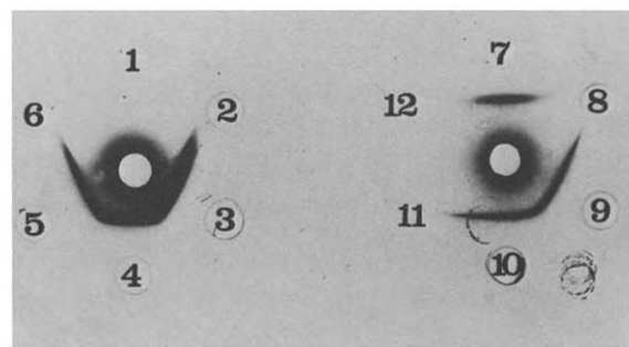
Fig.1. Ouchterlony analysis of monoclonal antibodies to rat liver epoxide hydrolase. The centre wells contained 10\text{ }\mu\text{g} epoxide hydrolase. The other wells contained the following ascites samples: (1) MZ-AD3 (clone B 8 ); (2) MZ-AD3 (clone G 8 ); (3) MZ-FC4 (clone B 1 ); (4) MZ-FC4 (clone B 8 ); (5) MZ-JC3 (clone E 1 ); (6) buffer; (7) MZ-HC3 (clone B 3 ); (8) MZ-HC3 (clone D 1 ); (9) MZ-JC3 (clone B 3 ); (10) MZ-JC3 (clone C 11 ); (11) buffer; (12) buffer.
